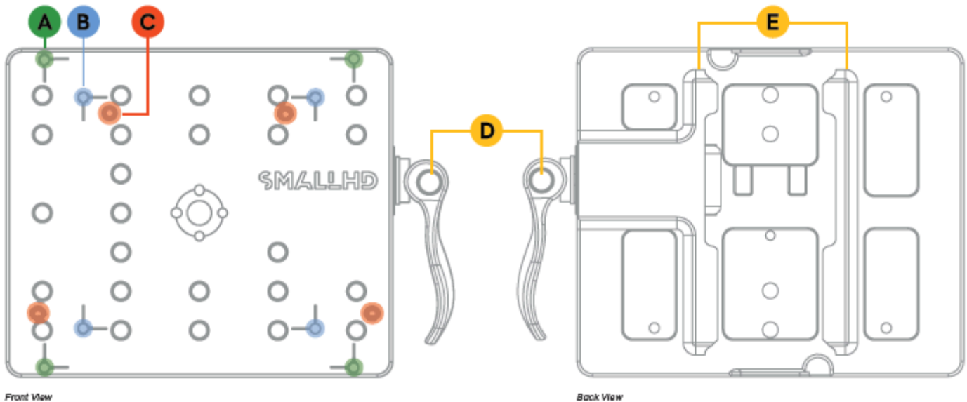
A. 100mm Mounting Pattern (4x M4-0.7 Holes)
